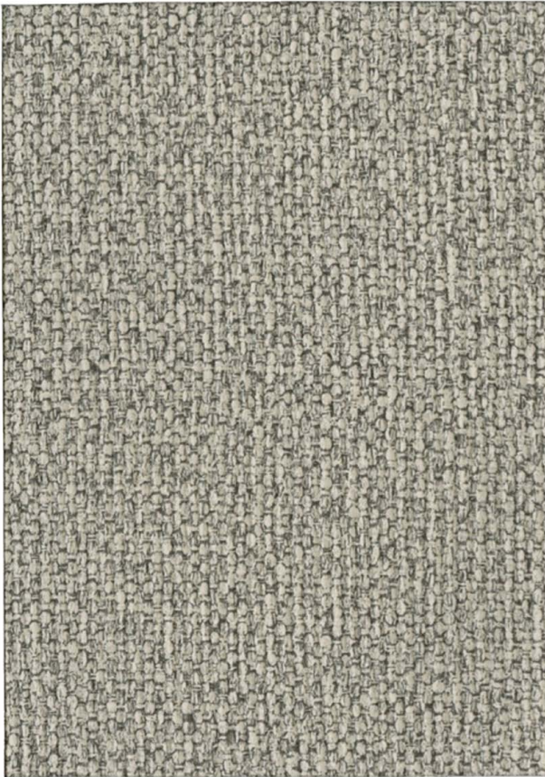
Smoke
